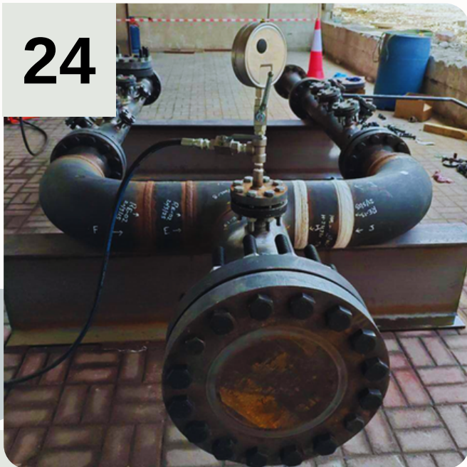
Skid piping
